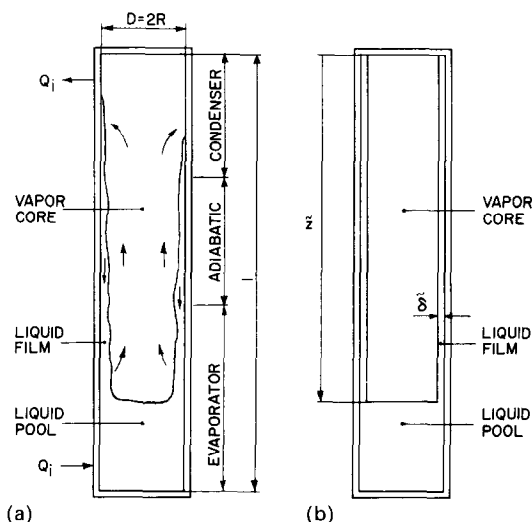
Fig. 1. (a) Actual two-phase flow in a thermosyphon; (b) idealized flow in a thermosyphon.
